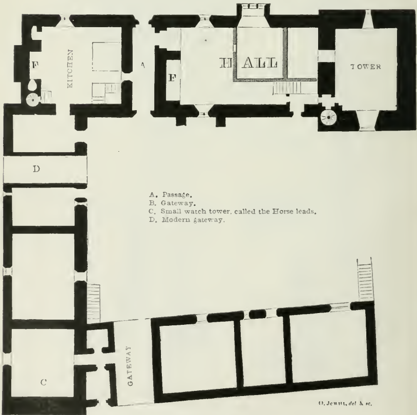
GROUND PLAN. YANWATH HALL, WESTMORELAND.
